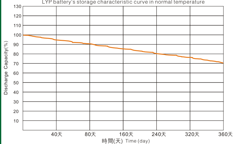
在常溫環境下LYP類電池的存儲特性曲線 LYP battery's storage characteristic curve in normal temperature
